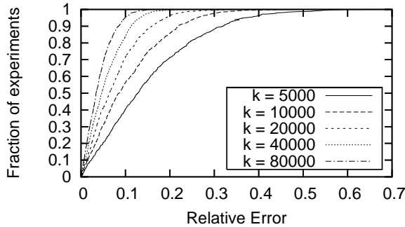
Figure 3: Varying numbers of buckets (Trace 2)
