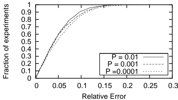
Figure 4: Varying sampling rates (Trace 2)
