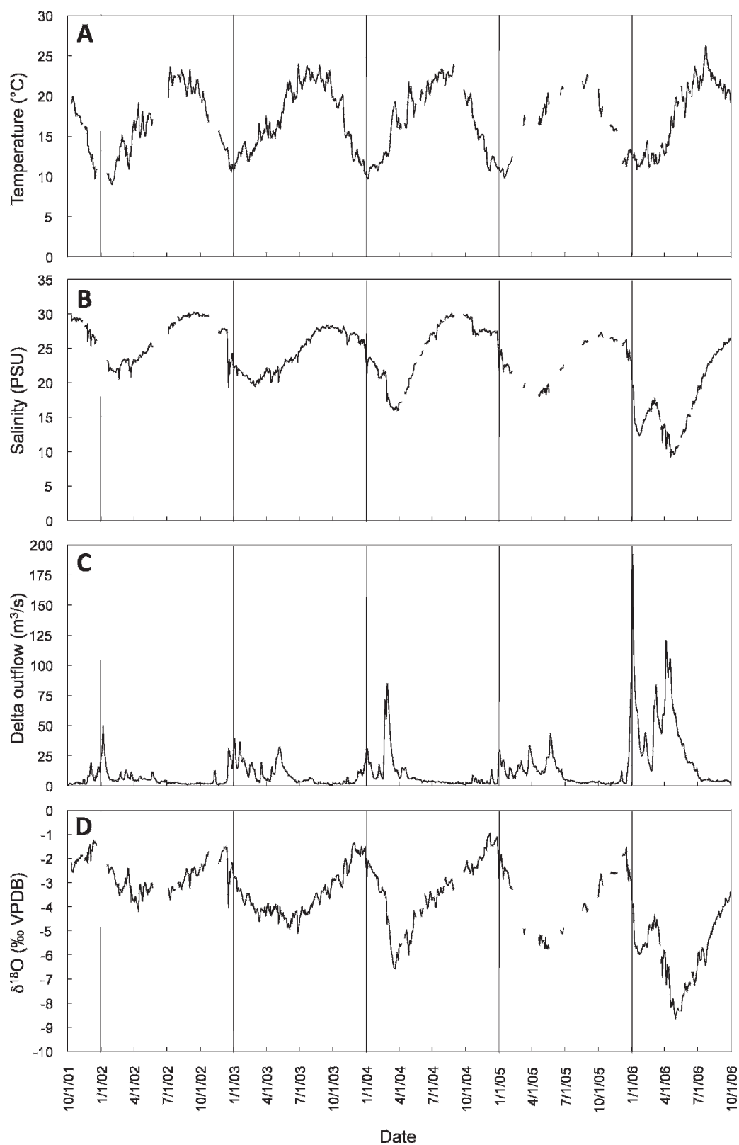
FIGURE 2 —Average daily temperature A) and salinity B) calculated from U.S. Geological Survey measurements at the end of the fishing pier adjacent to the east end of the Dumbarton Bridge; Delta outflow C) estimated by the California Department of Water Resources Interagency Ecological Program; and predicted oxygen-isotope profiles for mollusk shell calcite in south San Francisco Bay D). Vertical lines mark the beginning of each calendar year.
