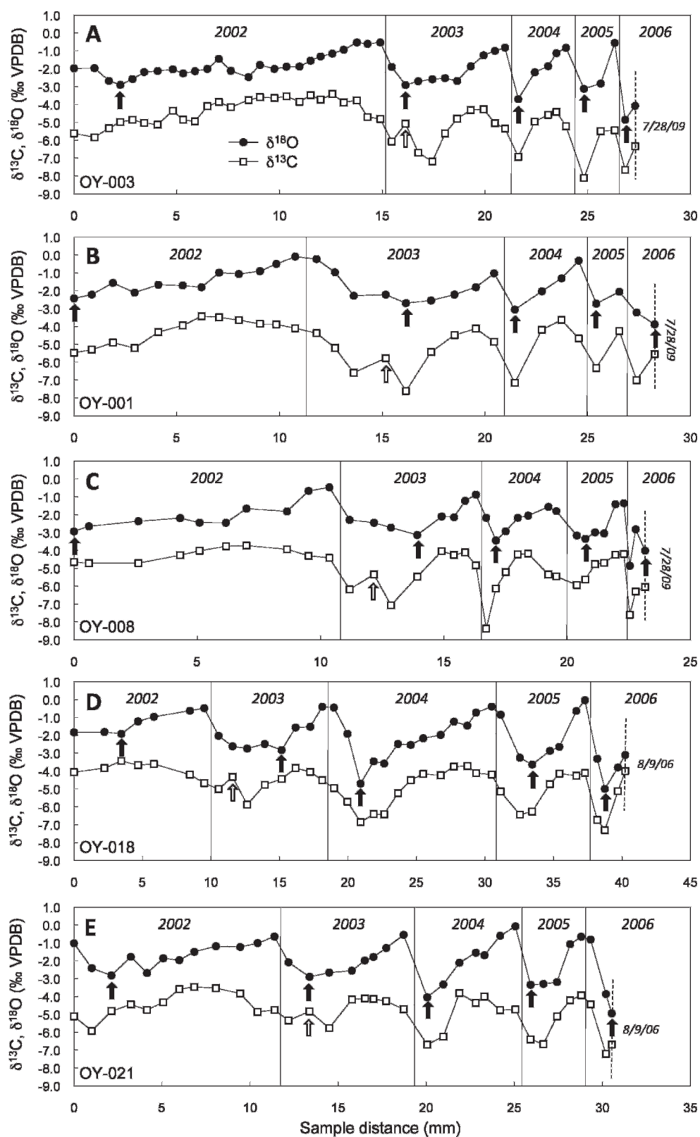
FIGURE 3 —Oxygen- and carbon-isotope profiles of five live Crassostrea gigas collected at Dumbarton Bridge and Hayward Landing in 2006 (Isotopic Pattern 1). Vertical dashed lines and dates near the right side of the graphs mark the collection dates. Vertical solid lines represent the approximate beginning of each estimated calendar year at the top of the graph, based on correlations with predicted \delta^{18}\text{O} values as described in the text. Filled arrows mark the end of each concave-down cycle and the open arrow marks the carbon spike.
