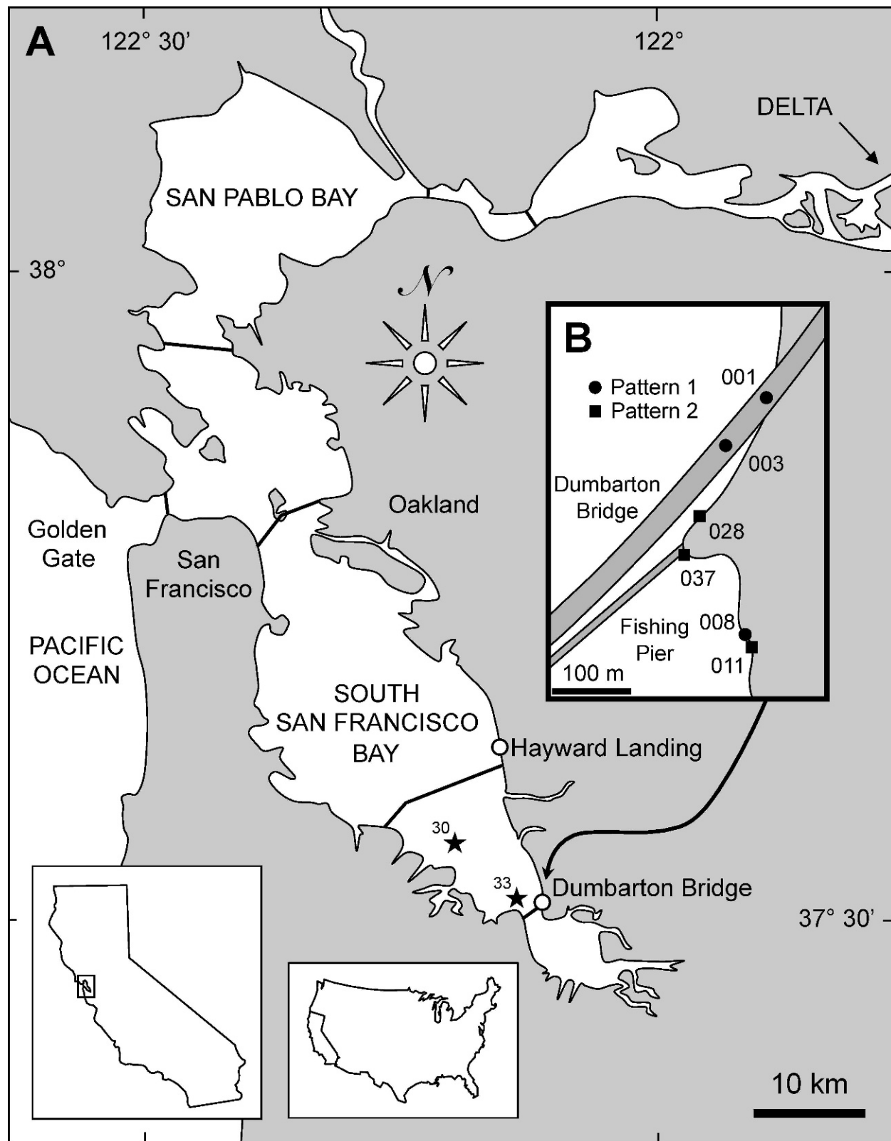
FIGURE 1—San Francisco Bay A) showing oyster shell collection sites = open circles; and chlorophyll sampling stations = stars. Heavy black lines mark the locations of bridges. B) Collection locations of Crassostrea gigas specimens from Dumbarton Bridge.
