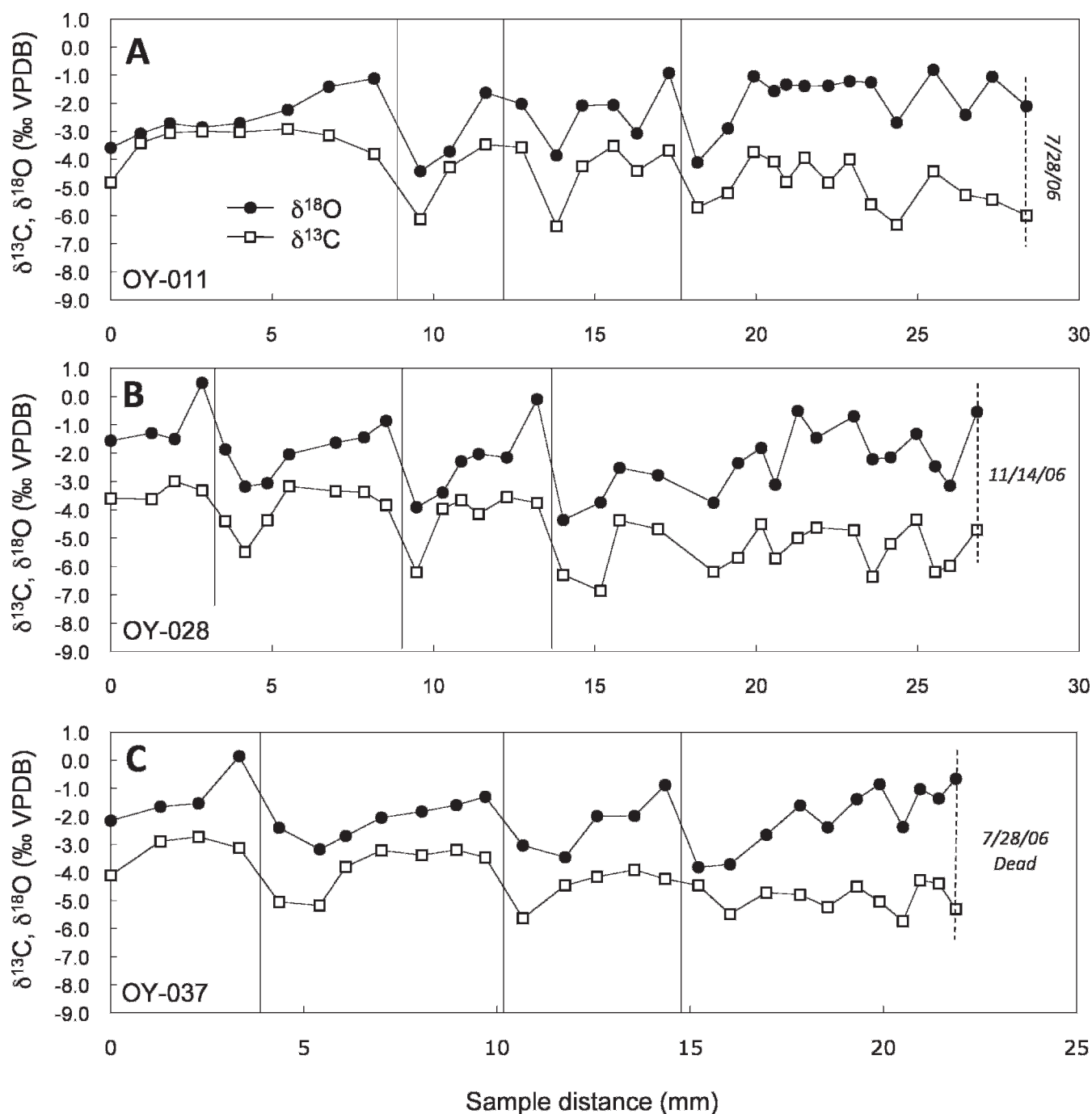
FIGURE 4 —Oxygen- and carbon-isotope profiles of two live Crassostrea gigas and one shell collected dead at Dumbarton Bridge in 2006 (Isotopic Pattern 2). Vertical dashed lines and dates near the right side of the graphs mark the collection dates. Vertical solid lines represent the approximate beginning of an estimated calendar year as described in the text.
