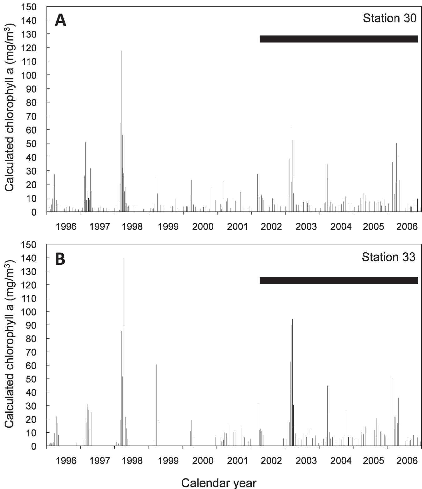
FIGURE 5 —Time series of calculated chlorophyll a concentrations from two sampling stations in the South Bay (see Fig. 1 for locations). Horizontal bars represent approximate lifespan of specimens in Group 1.
