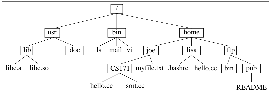
Figure 1: A simple example of a hierarchical file system.
